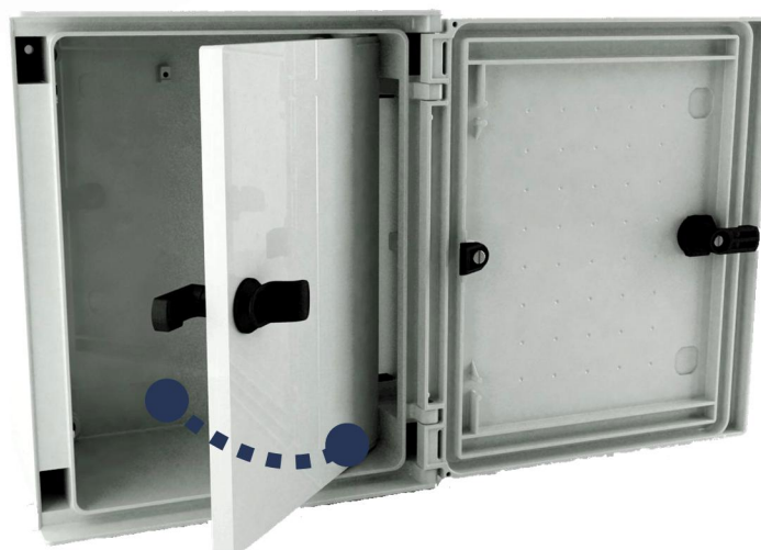
polyester internal door right opening, different lock options
