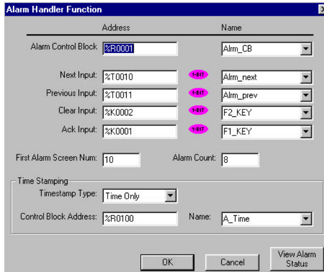
Figure 2.2 – Alarm Handler Function
