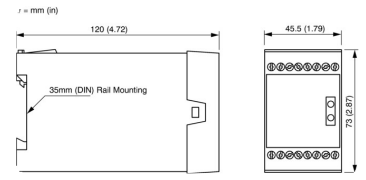
Sipha Control Unit Type 2
