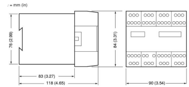
Sipha 6 Control Unit
