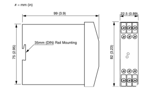
Sipha Control Unit Type 1
