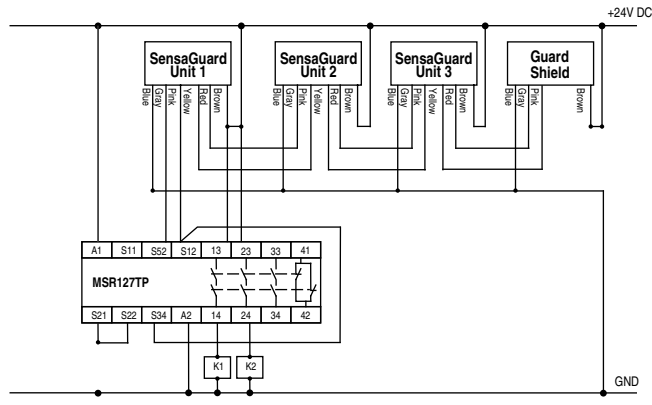
Automatic Reset
