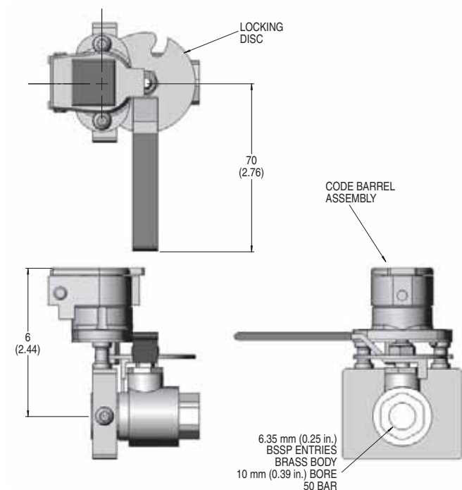
Approximate Dimensions [mm (in.)]
