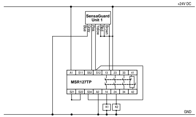
Automatic Reset
