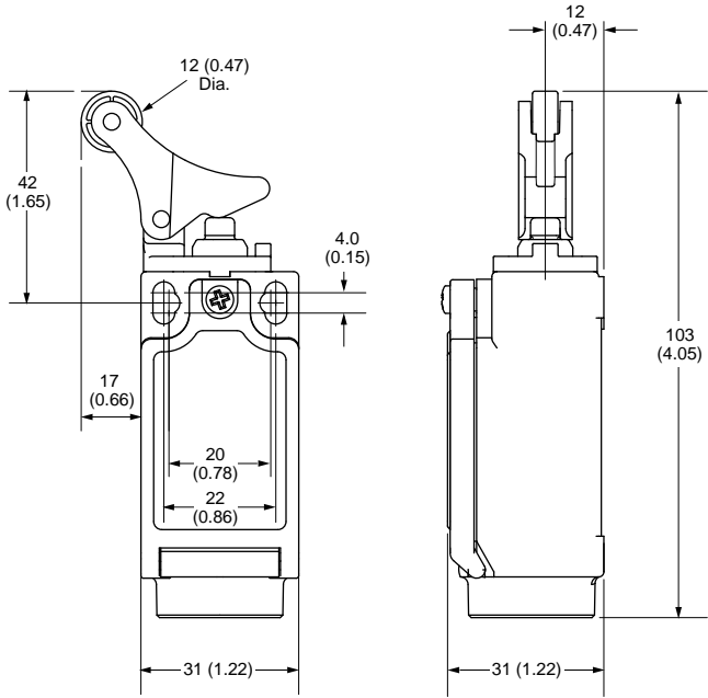
Offset Hinge
