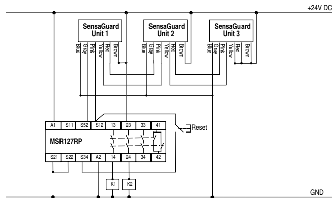
Monitored Reset
