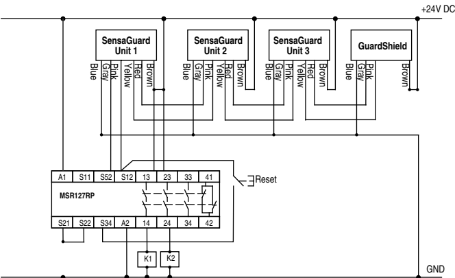
Monitored Reset
