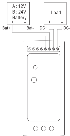
Fig 1.1 Suggested system connection
